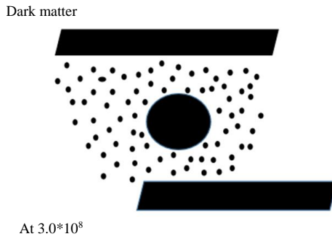
Fig. 1: “Dark matter” at the speed of light. Wave undergoing gravitational lensing. Gravity occurs in the y-direction
